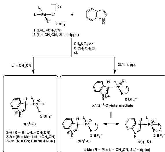
Scheme 2. Synthesis of dicationic indole-Pd II adducts. The \sigma(\eta^1-C) -mode of 3-H , 3-Me , and 3-Bn , and the \sigma/\pi(\eta^1-C) -mode for 4-Me were assigned.
