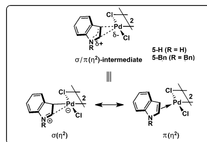
Scheme 3. Neutral indole-Pd II dichloride dimers 5-H and 5-Bn .
